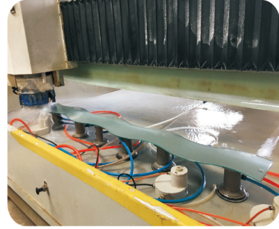
CNC machine
